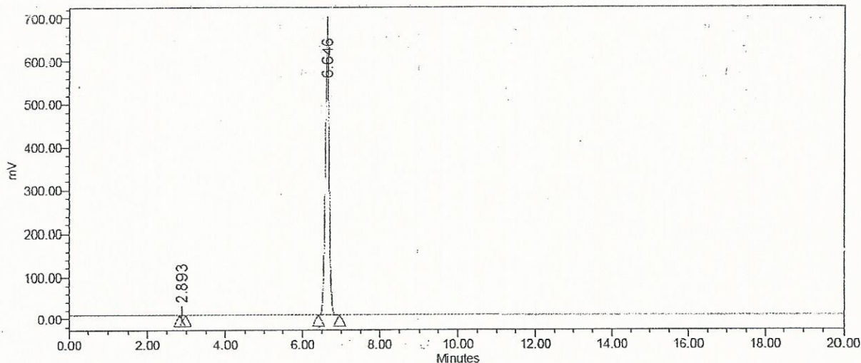
Auto-Scaled Chromatogram
